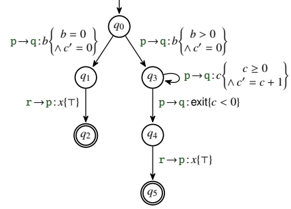
Figure 10: Example where states q_1 and q_3 violate Send Coherence for r .
