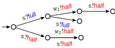
Figure 3: Local implementation for w_1
