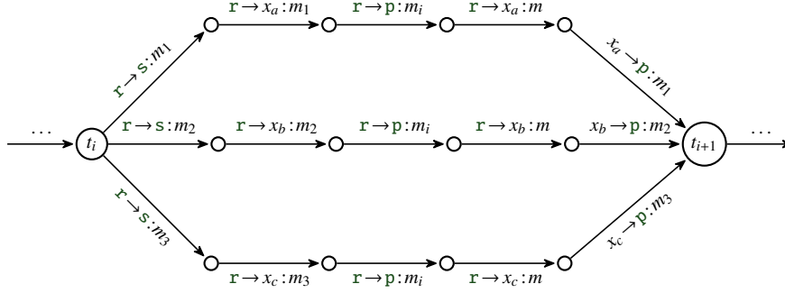
Figure 7: Clause selection gadget \mathcal{S}_C .
