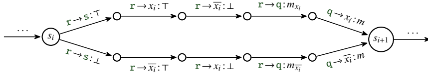
Figure 6: Variable assignment gadget \mathcal{S}_X .
