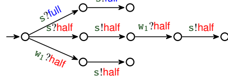
Figure 4: Local implementation for w_2
